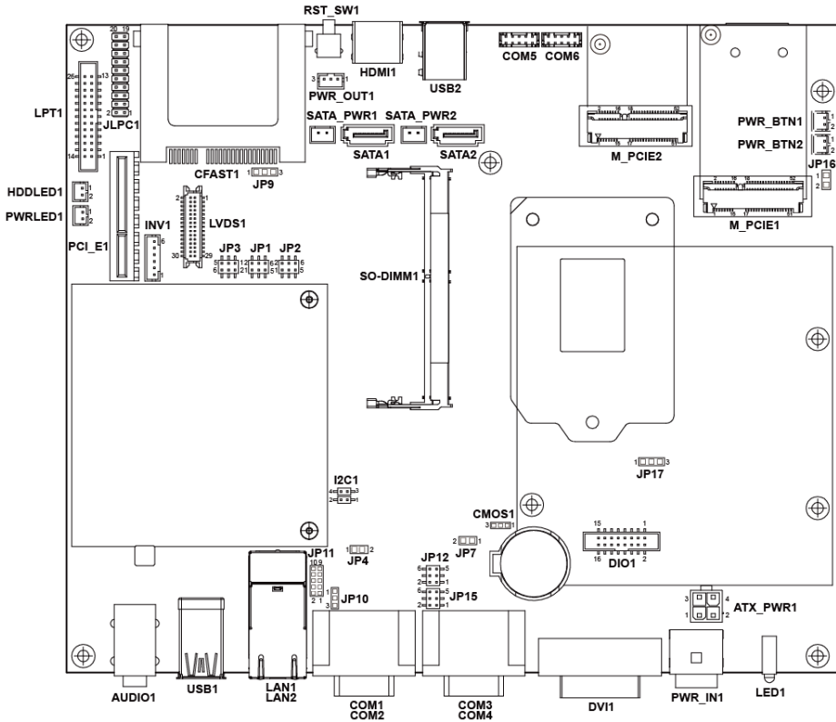
Figure 3-1. Main Board Component Location (Top View)
